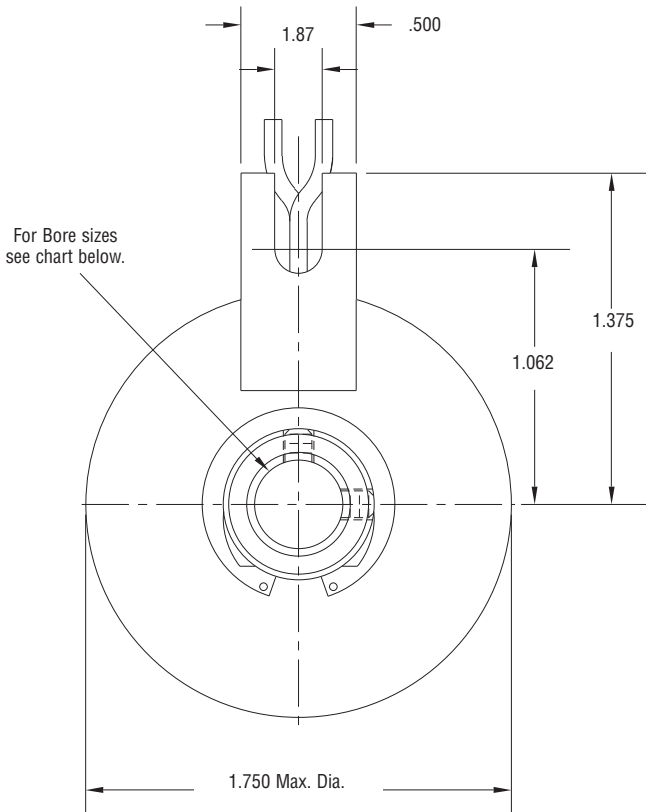
FIELD VIEW
