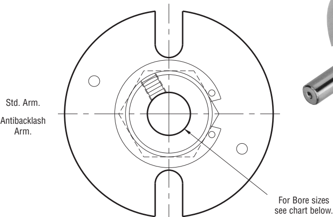
ARMATURE VIEW
