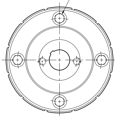
ARMATURE VIEW
