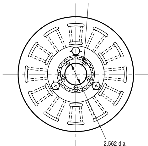
ARMATURE VIEW
