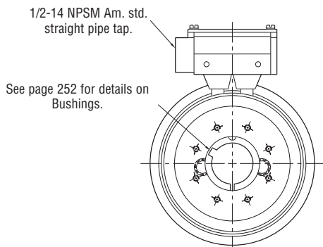
COLLECTOR RING VIEW
