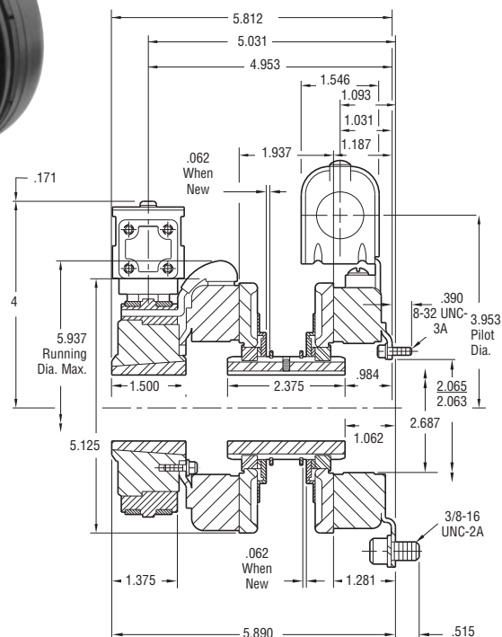
Outside Mounted Offset Backing Plate
