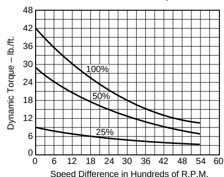
Size 500-PC/PB Maximum Speed 5,400 rpm Static Torque 40 lb./ft.
