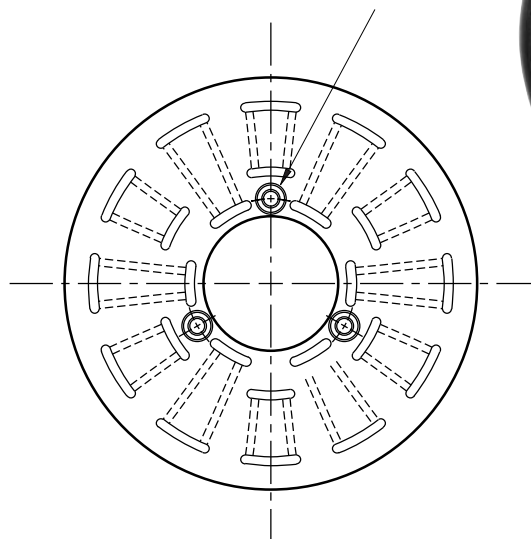
ARMATURE VIEW
