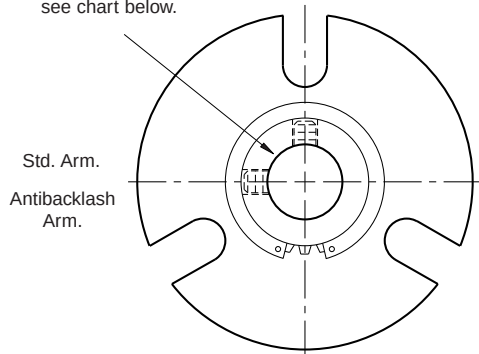
ARMATURE VIEW
