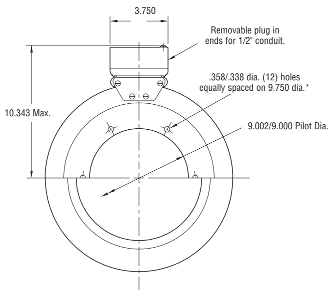
MAGNET VIEW
