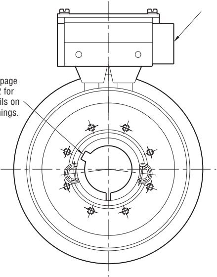
MAGNET VIEW
