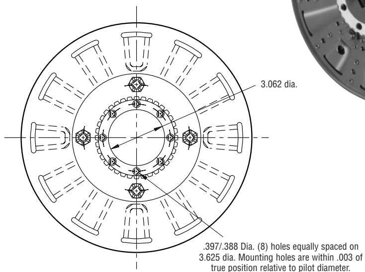
ARMATURE VIEW
