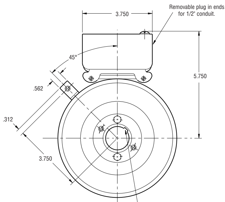
ARMATURE VIEW
