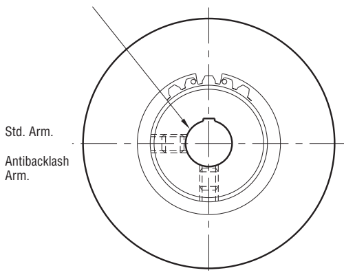
ARMATURE VIEW
