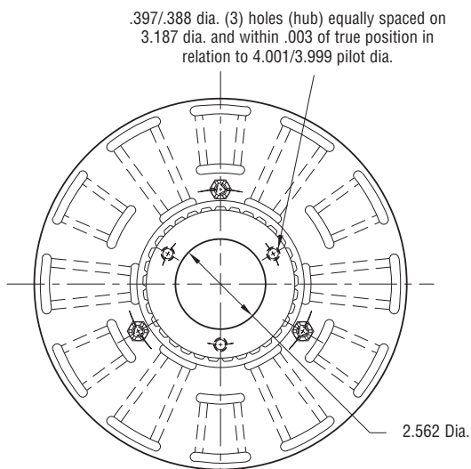
ARMATURE VIEW
