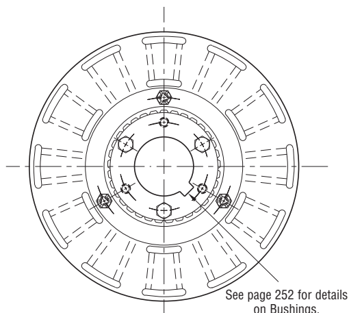
ARMATURE VIEW
