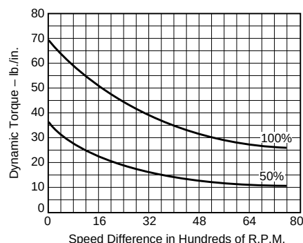
Size 250 Maximum Speed 7,500 rpm Static Torque 70 lb./in.
