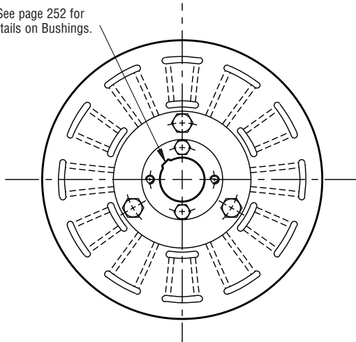
ARMATURE VIEW
