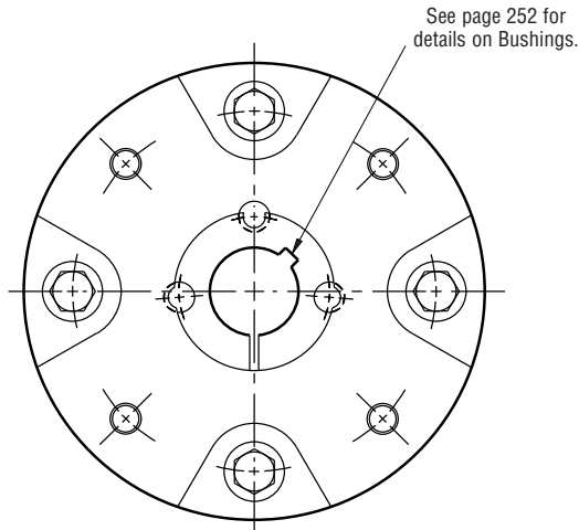
HUB VIEW
