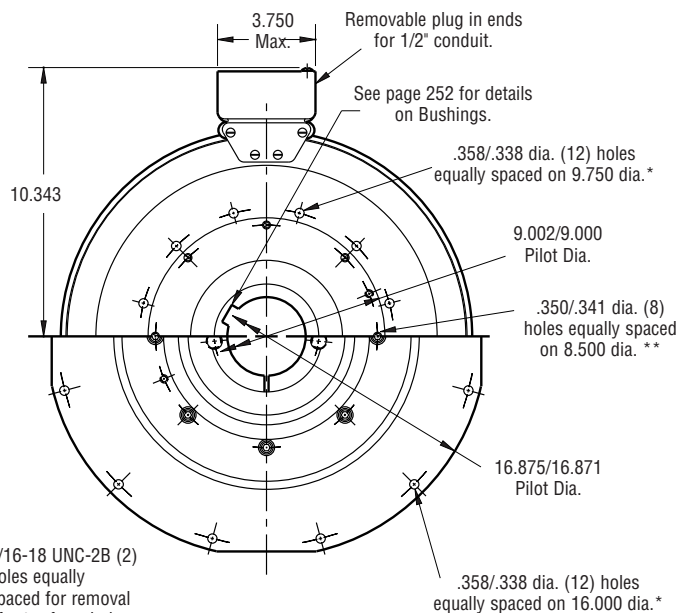
FIELD VIEW
