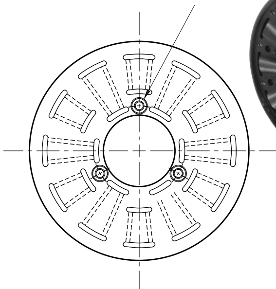
ARMATURE VIEW
