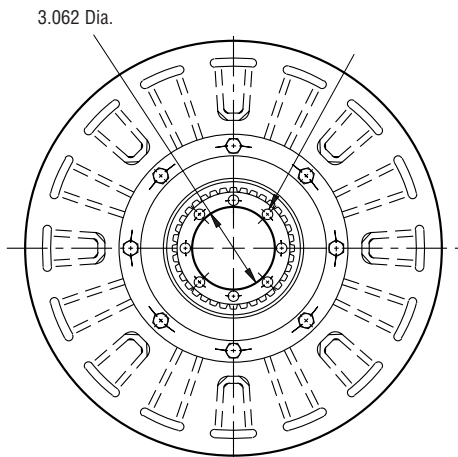
ARMATURE VIEW
