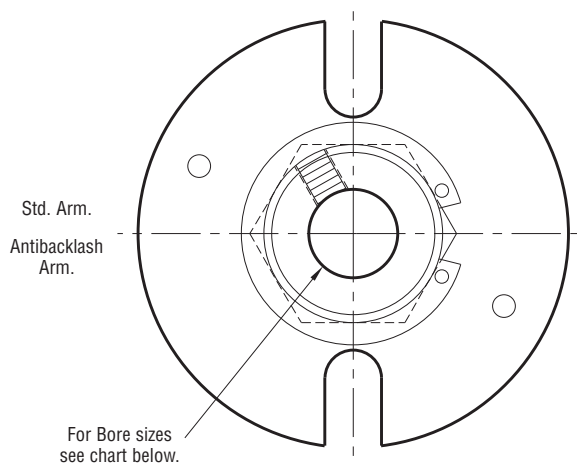
ARMATURE VIEW
