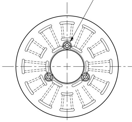
ARMATURE VIEW
