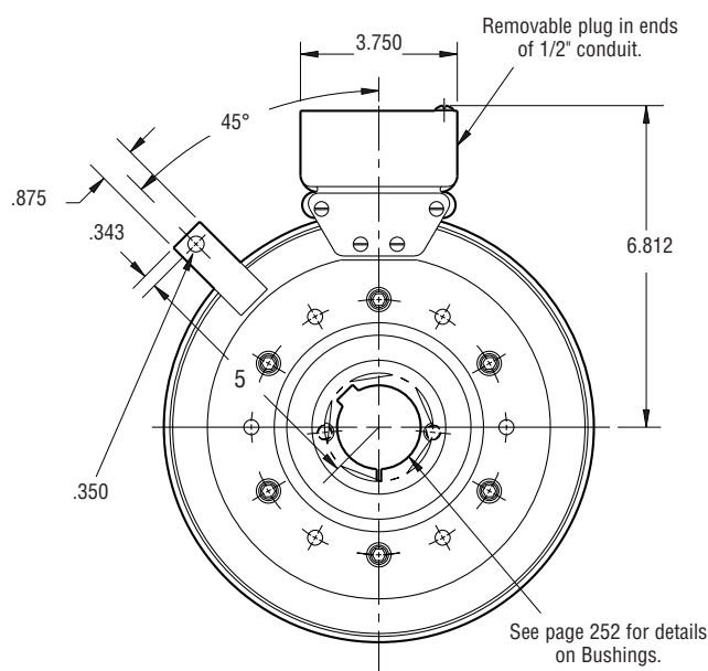
FIELD VIEW
