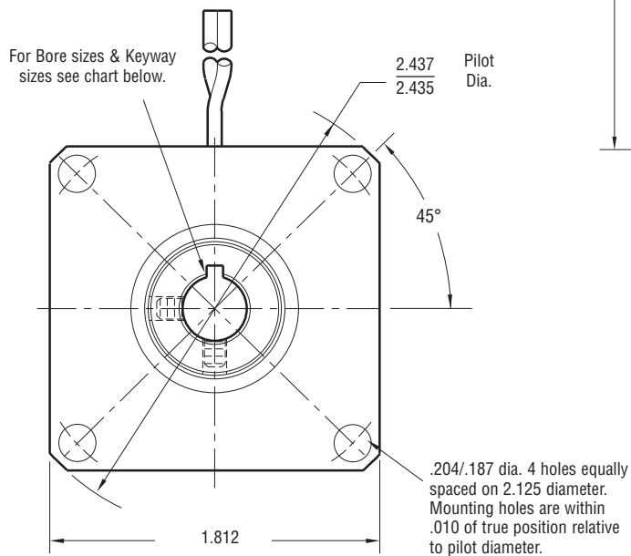
FIELD VIEW
