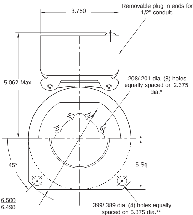
MAGNET VIEW
