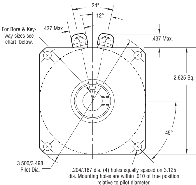
FIELD VIEW
