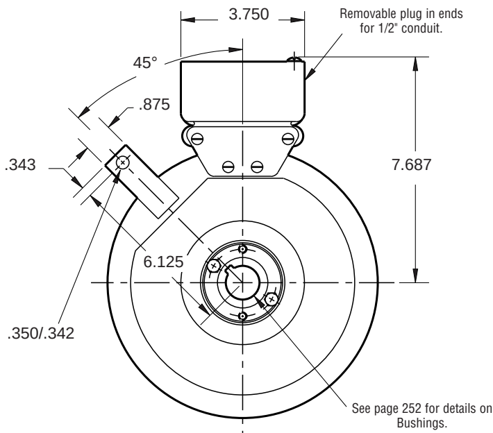
FIELD VIEW
