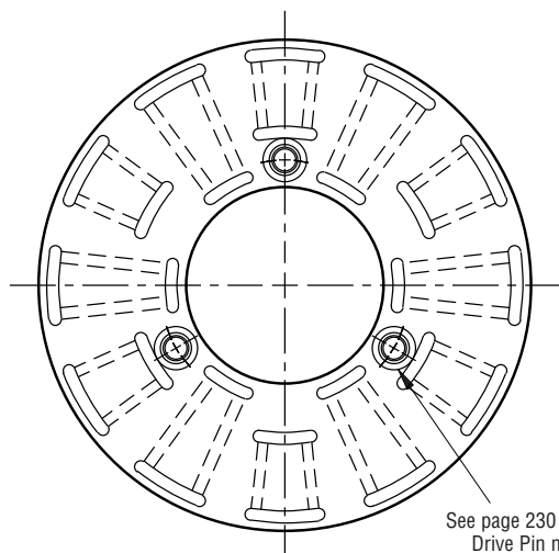
ARMATURE VIEW
