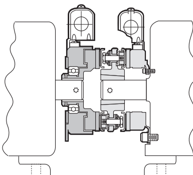
SFPBC Clutch/Brake Coupling Typical Installation
