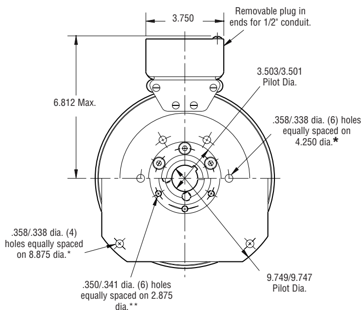
FIELD VIEW
