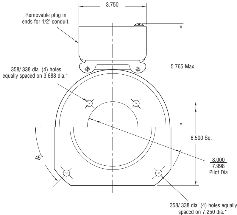
MAGNET VIEW
