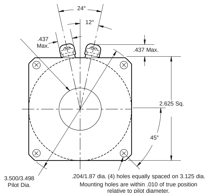
FIELD VIEW
