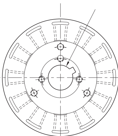
ARMATURE VIEW
