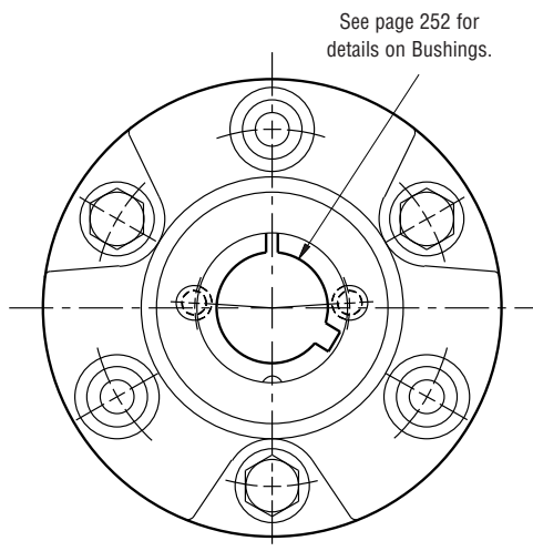
HUB VIEW
