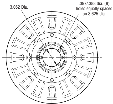
ARMATURE VIEW
