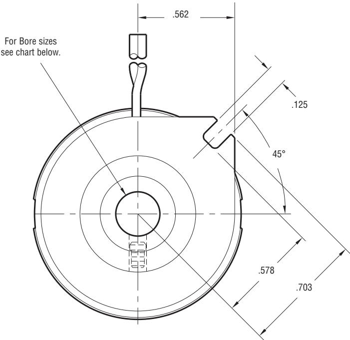
FIELD VIEW
