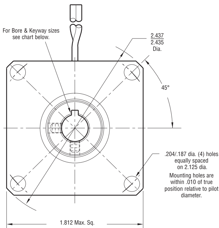
FIELD VIEW
