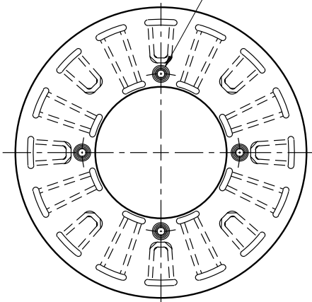
ARMATURE VIEW
