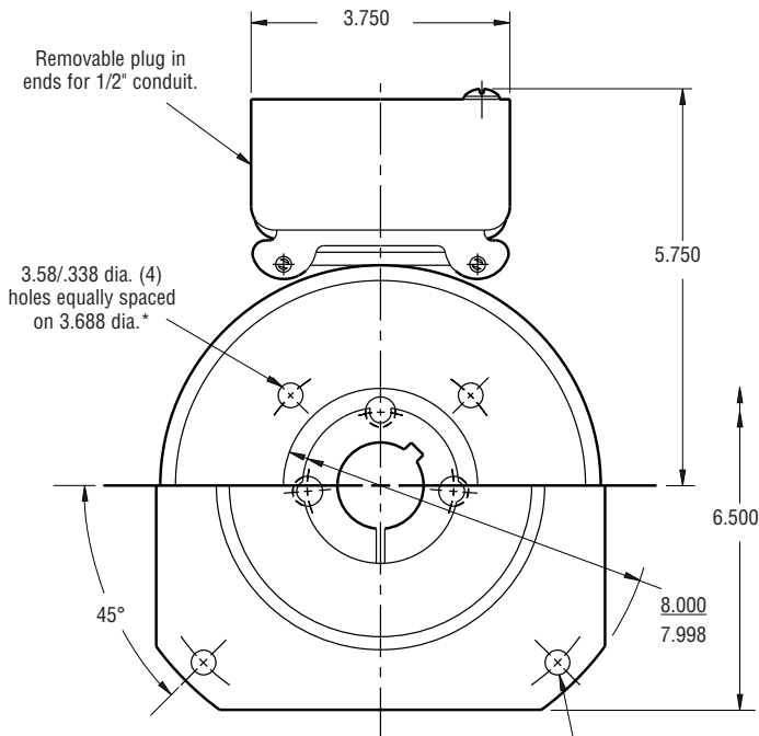
HUB VIEW
