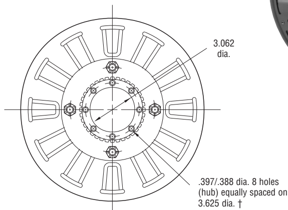
ARMATURE VIEW
