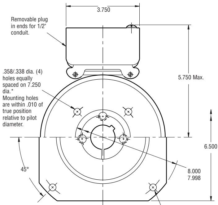
ARMATURE VIEW
