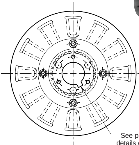
ARMATURE VIEW
