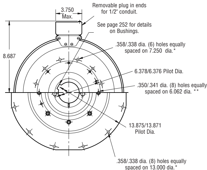
FIELD VIEW
