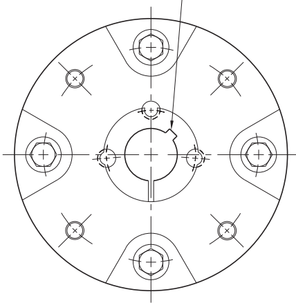
HUB VIEW
