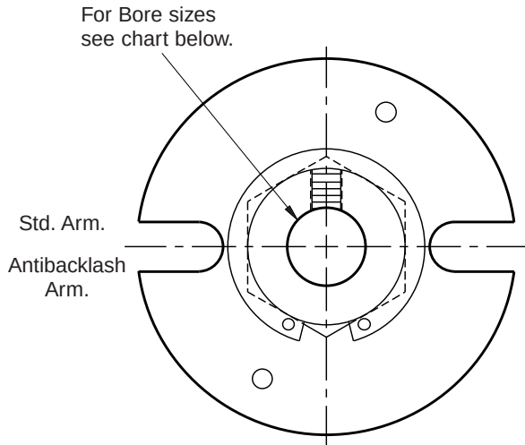
ARMATURE VIEW
